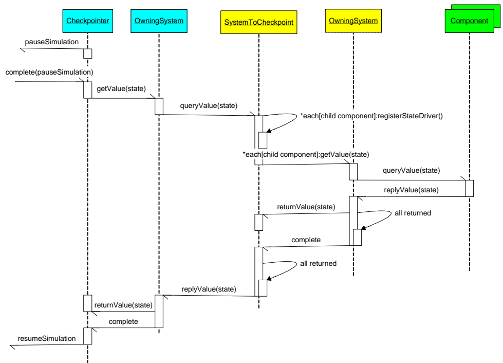
Checkpointing
